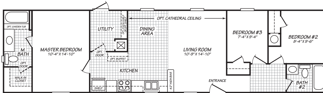
ALTERNATE #1 - 4' STRETCH - 3 BEDROOMS
